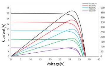
I-V/P-V Curve at Different Irradiation SSA-54HDB-495N
