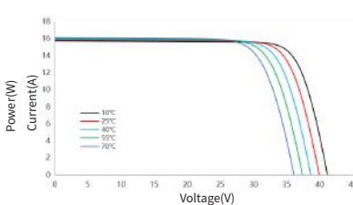
I-V Curve at Different Temperature SSA-54HDB-495N
