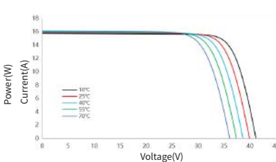
I-V Curve at Different Temperature SSA-54HD-495N
