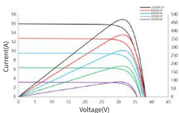
I-V/P-V Curve at Different Irradiation SSA-54HD-495N
