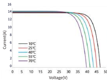
I-V Curve at Different Temperature SS8-66HD-505M
