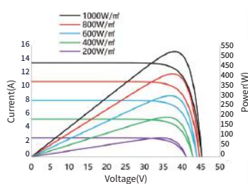
I-V/P-V Curve at Different Irradiation SS8-66HD-505M
